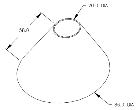
DISCHARGE END BMH DISCHARGE HOPPER LINER 1" THICK - BHM-001
